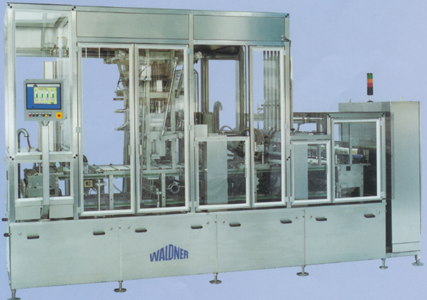
DOSOMAT 20.4 with laminar airflow cabinet
